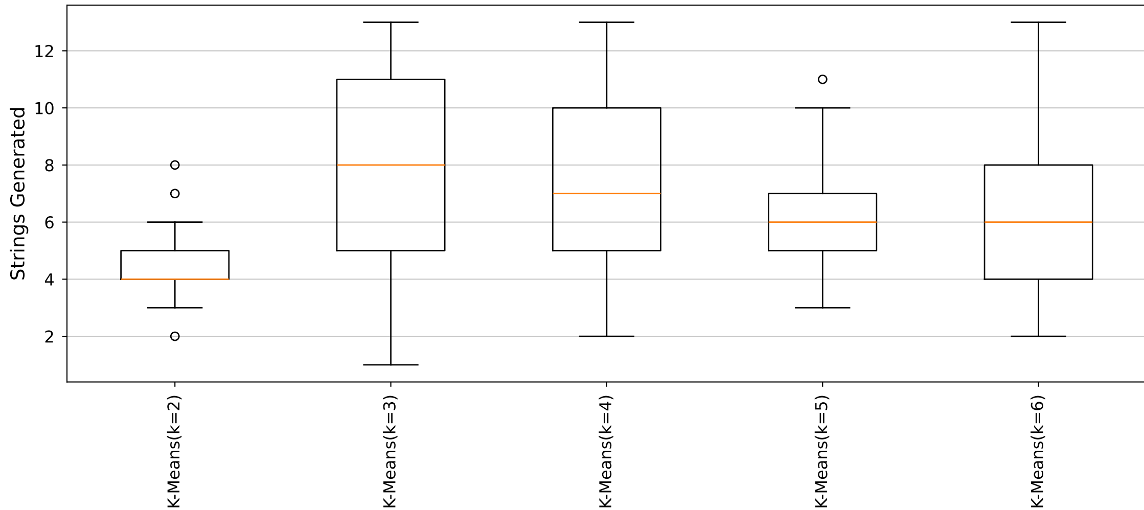
YARA Rules Strings Generated Distribution (Cluster31_Size6 dataset)
